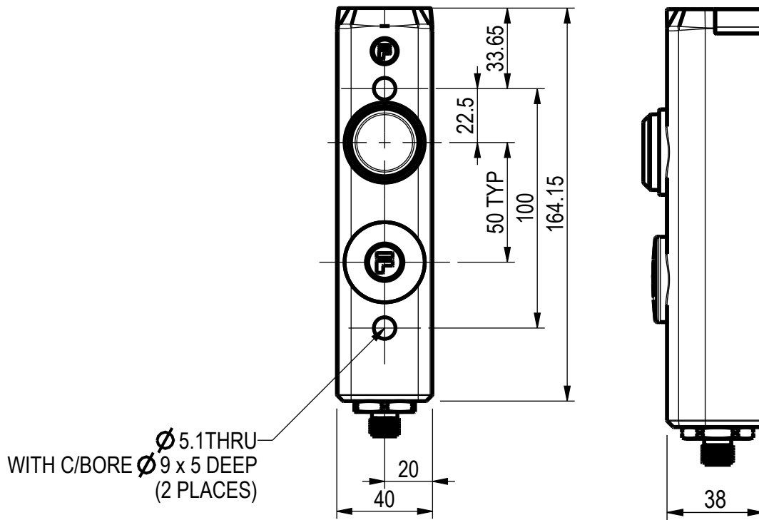
Figure 2: Dimensional Drawing - TLB, TLG, TLR, TLW, TLY
